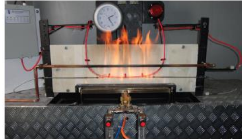
Fire with mechanical shock IEC 60331
